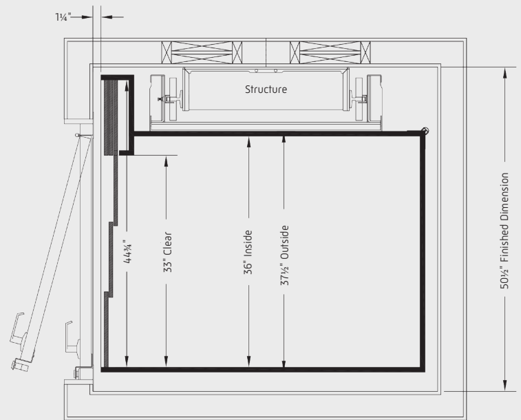
Shown with Symmetry Flush Mount Landing Door Package
